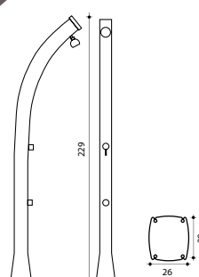
Green DS-H422VE
